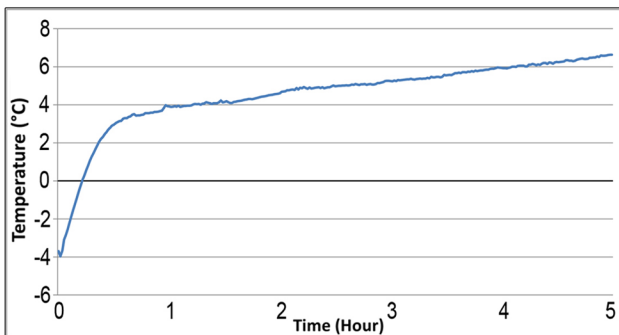
CryoCommand PL6 Sample Temperatures: CL Cryo-Core
